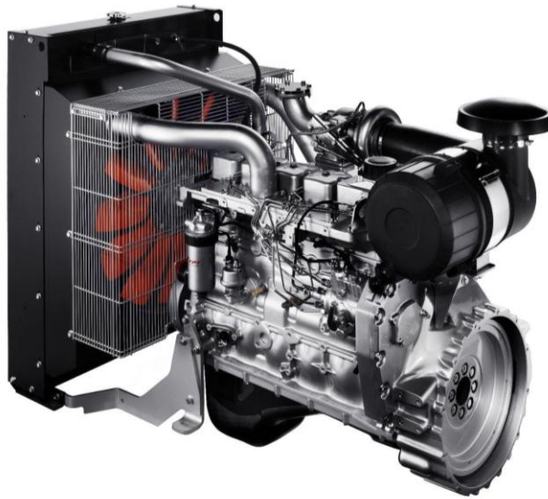
Motor FPT Industrial N67 TM6
